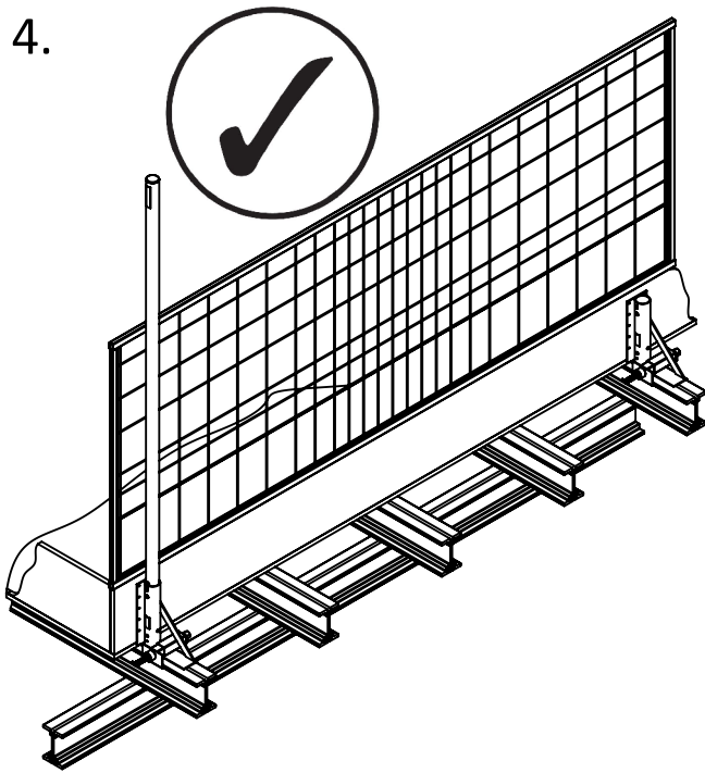
Correct orientation of Barrier
