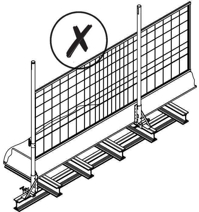
Incorrect orientation of Barrier
