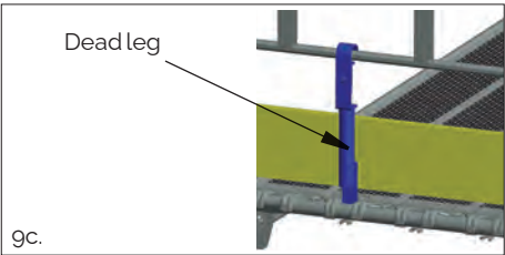
9c. Scaffold boards with HAKI Dead Leg.
